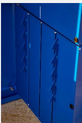
Retainers to prevent spring back of material in the bale chamber
